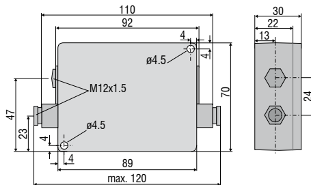
Controller
