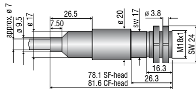
Sensor
