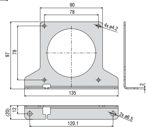
WPS-MB88 for the MK88 series
