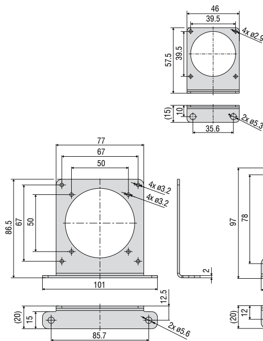
WPS-MB77 for the MK77 series
