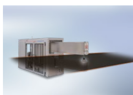
Robust system for thickness measurement (up to 5 measurement tracks) thicknessCONTROL BTG 8702 C.C
